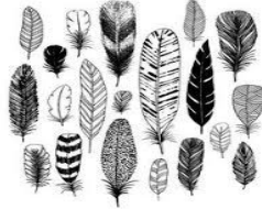
Plumes
